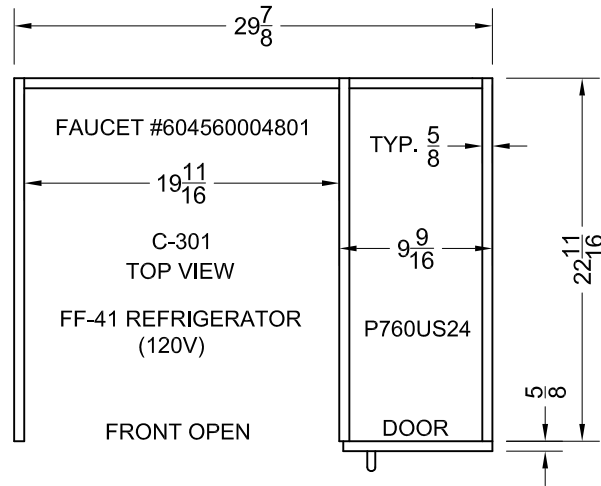
ALL-IN-ONE KITCHEN C-301
